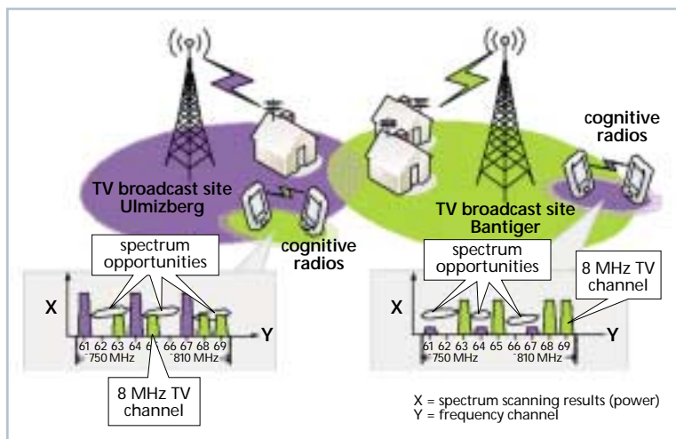
Fig. 3. Cognitive radio in the TV band: At different locations, the cognitive radio devices detect different frequency channels as free and interpret them as opportunities for their own communication. This example for vertical spectrum sharing is discussed at IEEE 802.22™ standardisation.
