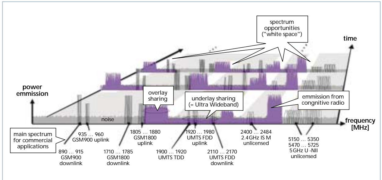
Fig. 2. Opportunistic spectrum usage by cognitive radios in a wide range of frequencies.
