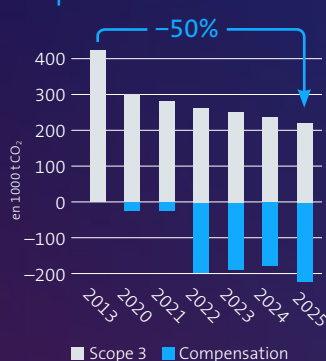
Scope 3
