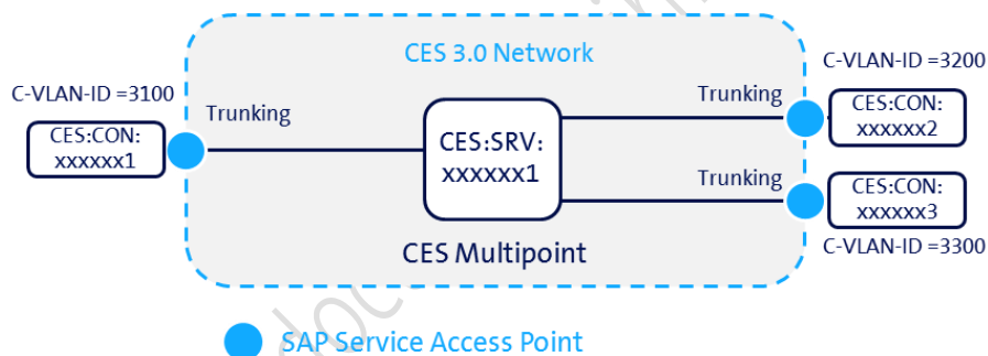
Figure 10: VLAN ID maintenance EVPx
