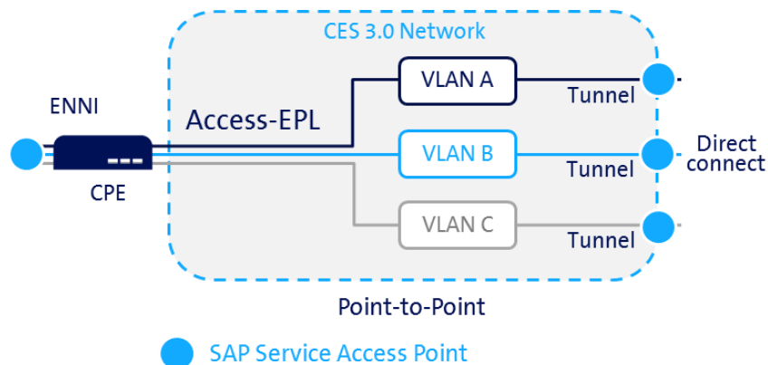
Figure 6: Access-EPL with "Tunnel - ENNI" configuration
