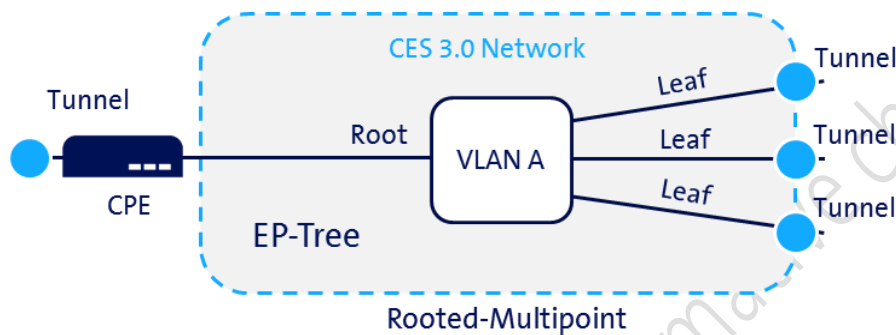
Figure 5: EP-Tree with "Tunnel – Tunnel" configuration
