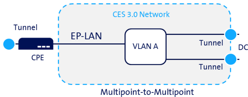
Figure 4: EP-LAN with "Tunnel – Tunnel" configuration
