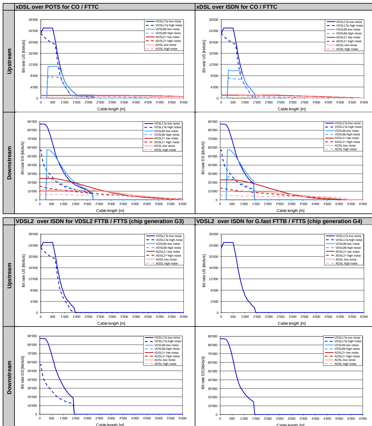
Figure 2: xDSL over POTS reference bit rate performance curves; for numeric values, cf. Sections 7.8 to 7.11.
