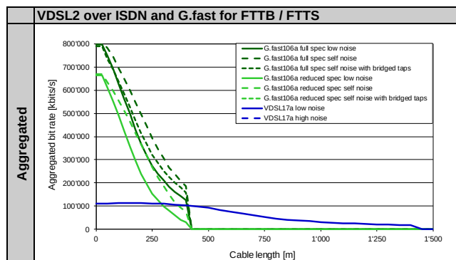
Figure 3: VDSL2 over ISDN and G.fast reference bit rate performance curves; for numeric values, cf. Section 7.8,
