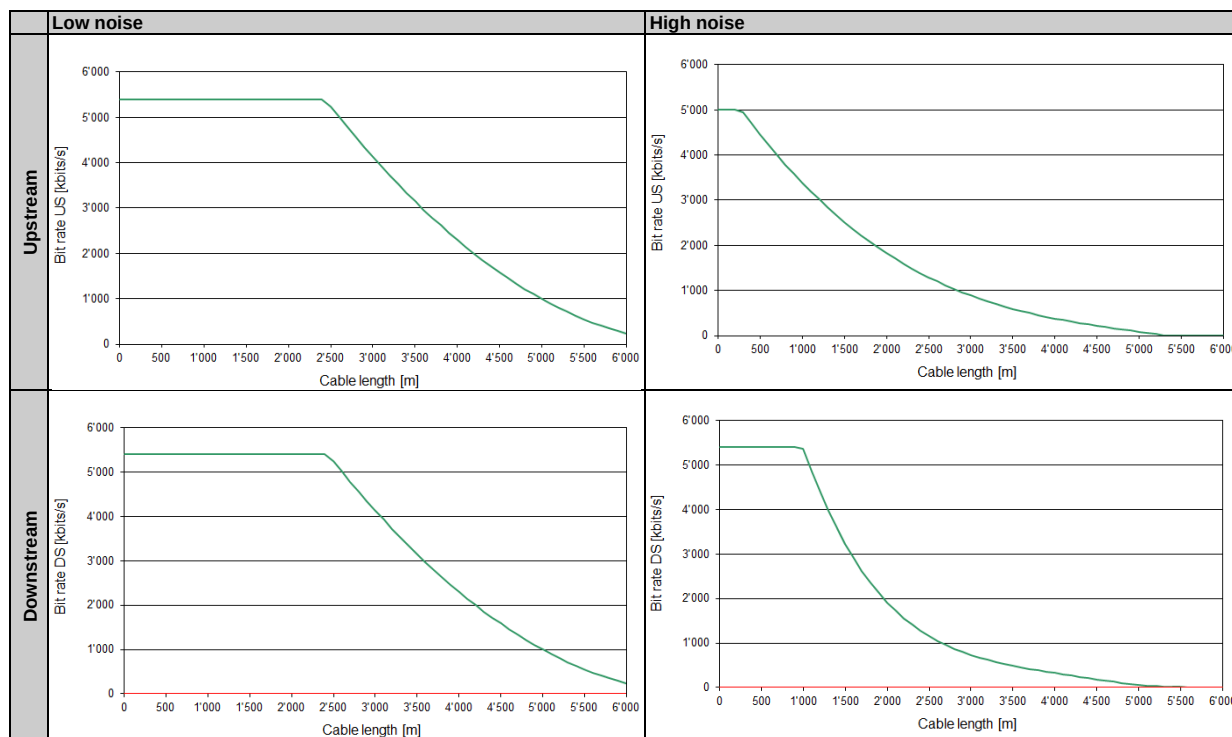
Figure 4: SDSL reference bit rate performance; for numeric values, cf. Section 7.12.
